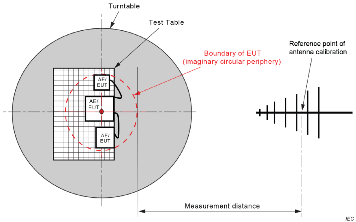
Figure C.1 – Measurement distance
